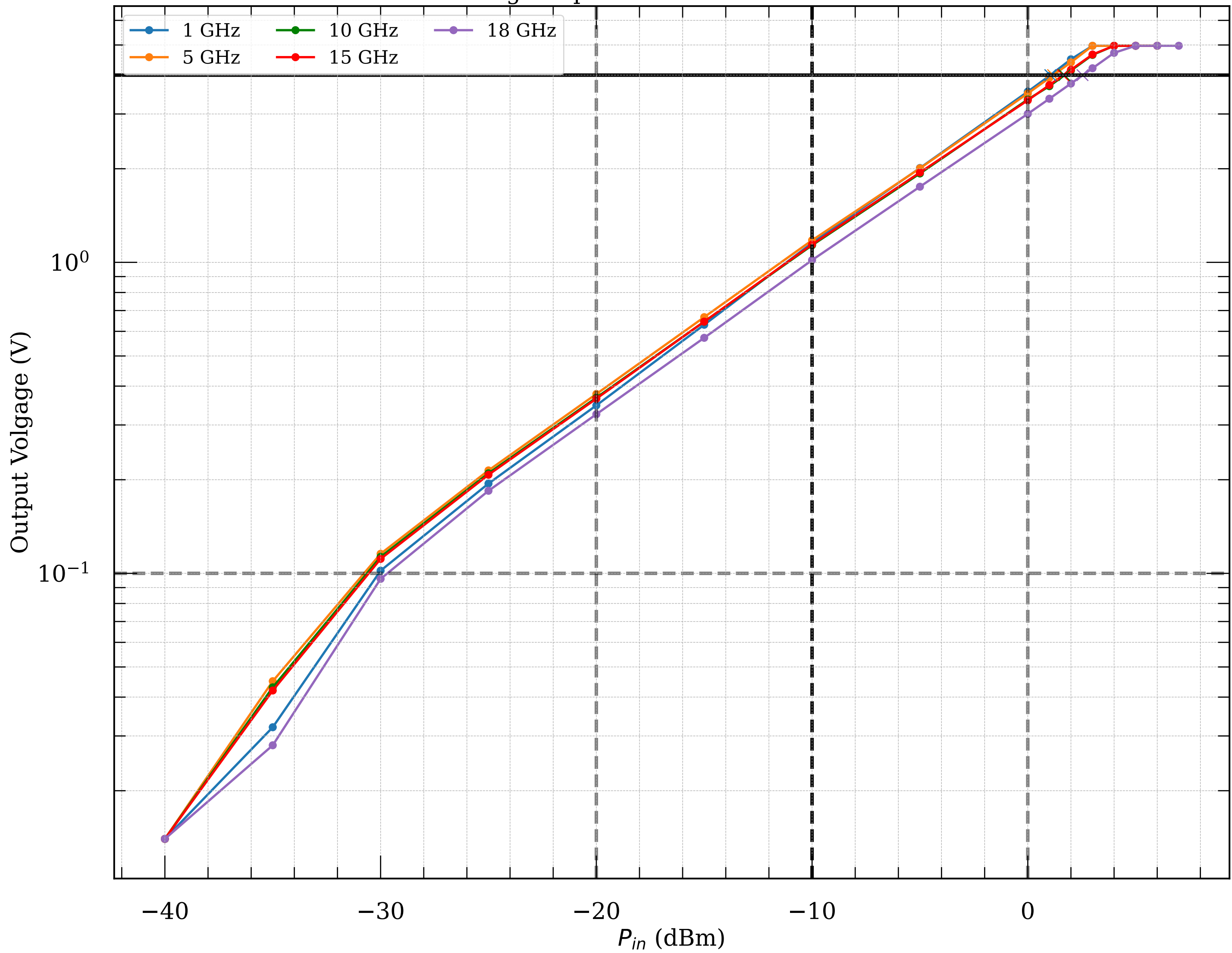
Measured voltage-to-power curve of detector module005v2
